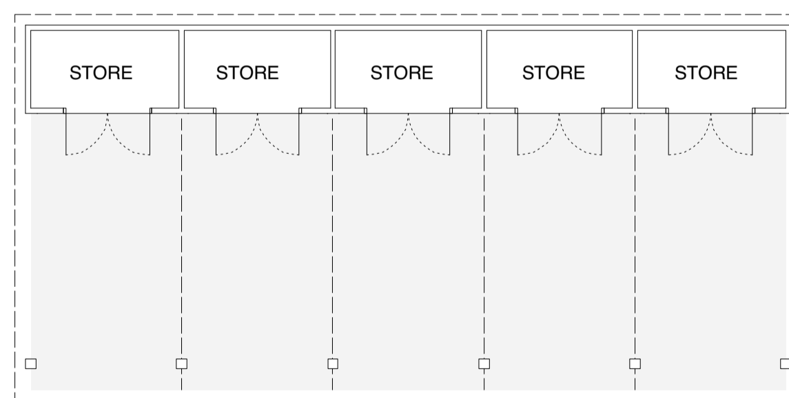
Carport B Plan Scale 1:100 @ A1
